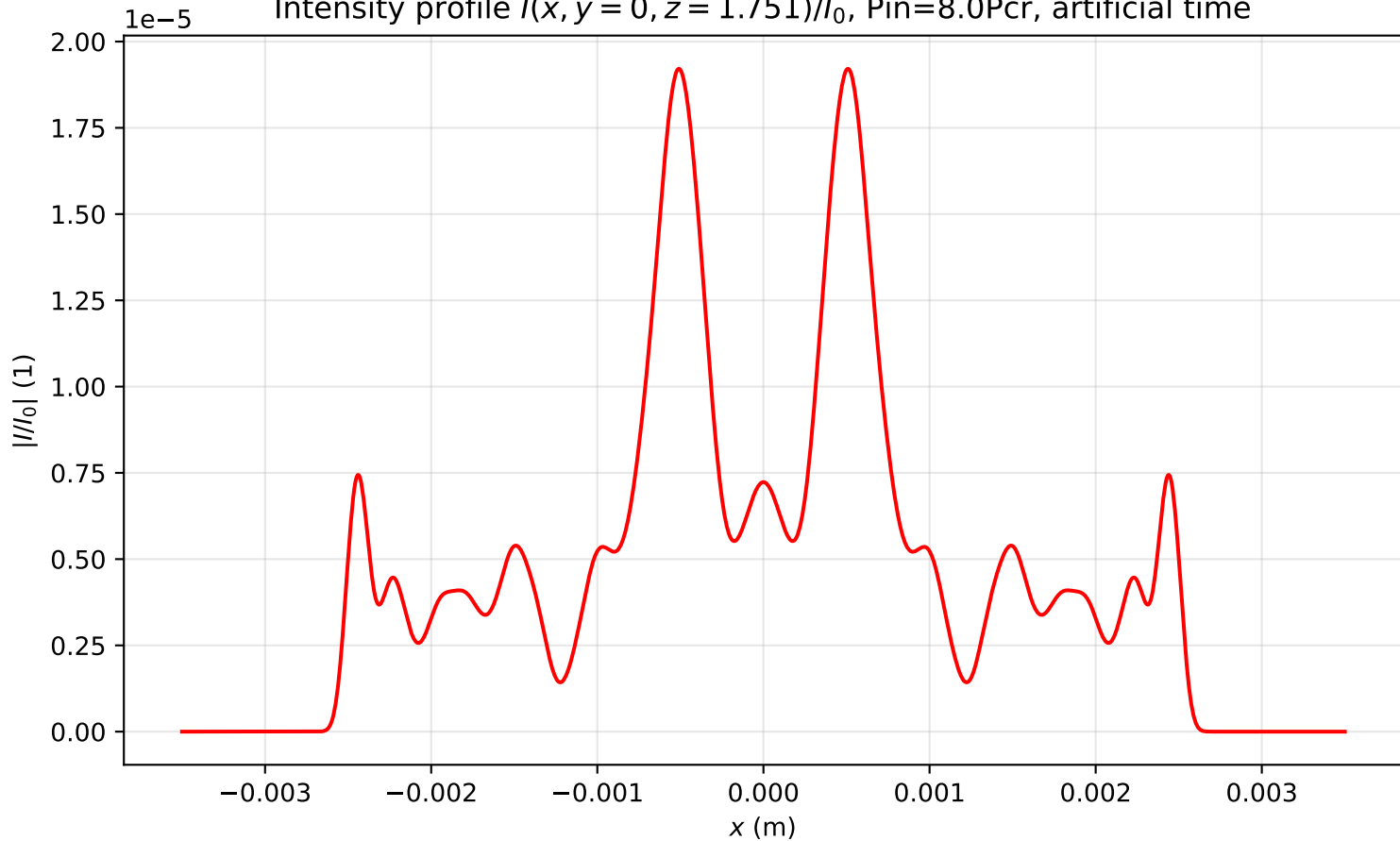
Intensity profile I(x, y = 0, z = 1.751)/I_0 , P_{in}=8.0P_{cr} , artificial time
